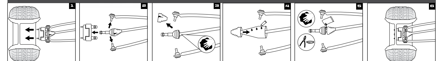
1 Remove wheel and axle nut 2 Remove brake caliper, hub, tie rod, & upper & lower ball joints 3 Remove old boot & clean joint 4 Spread silicone lube on entire cone tool. Slide boot over cone tool, large end first. See package for outer boot instructions. 5 Empty the bag of grease into the CV joint/boot, clean sealing points & install clamps 6 Reassemble tie rod, ball joints, brake caliper, axle nut, tire & wheel
