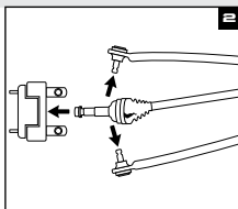
Remove brake caliper, hub, tie rod, & upper & lower ball joints.
