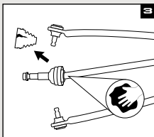
Remove old boot & clean joint.
