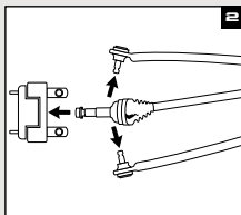
Remove brake caliper, hub, tie rod, & upper & lower ball joints.
