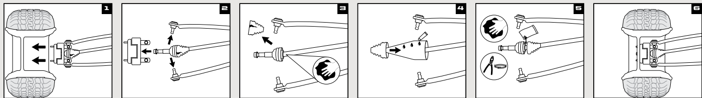
Remove wheel and axle nut. Remove brake caliper, hub, tie rod and upper and lower ball joints. Remove old boot and clean joint. Spread silicone lube on entire cone tool. Slide boot over cone tool, large end first. See package for outer boot instructions. Empty the bag of grease into the CV joint/boot, clean sealing points and install clamps. Reassemble tie rod, ball joints, brake caliper, axle nut, tire and wheel.
