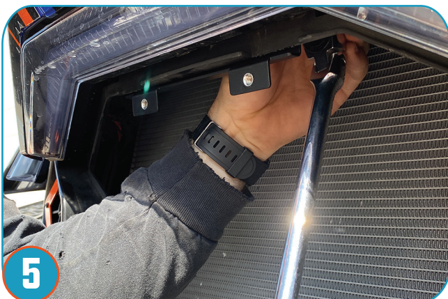
5 USING THE 2-NUTS REMOVED IN STEP 4, PLACE PROVIDED GRILLE BRACKET AND RE-APPLY NUTS TO SECURE BRACKET IN PLACE (DO NOT OVER-TIGHTEN).
