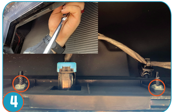
4 REMOVE THE TWO NUTS INSIDE AND ABOVE THE RADIATOR SCREEN USING A 11MM SOCKET.
