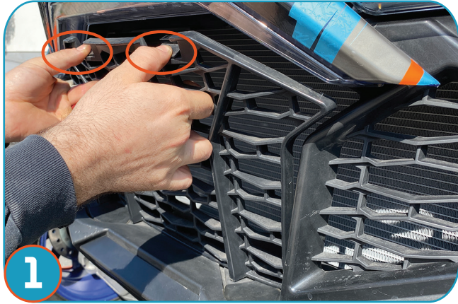
1 REMOVE FRONT OEM GRILLE FROM YOUR VEHICLE, PRESSING DOWN ON TWO TABS.
