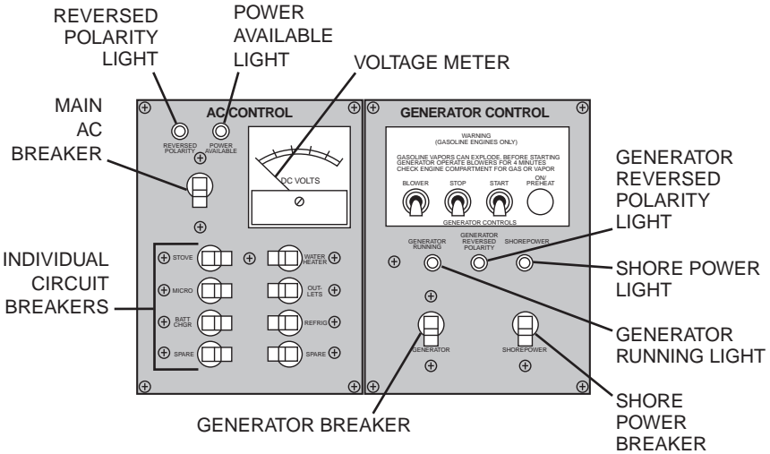
TYPICAL AC/GENERATOR CONTROL PANEL
