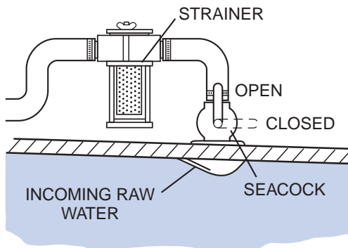
TYPICAL SEACOCK AND STRAINER
