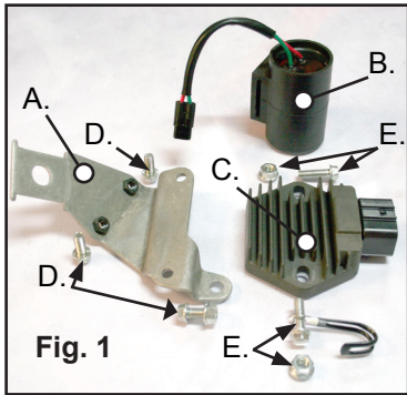
OEM Reg/Rec and Capacitor removed
